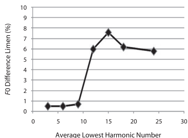
Figure 12. The threshold change in fundamental frequency ( F_0 difference limen) in percentage of f_0 , required to discriminate a change in F_0 as a function of the lowest component (lowest harmonic) in a 200-Hz-fundamental complex harmonic sequence. There is a large decrement in performance when the harmonic number is approximately the 10th. This loss in performance might be due to a lack of resolvable harmonics above the 10th harmonic. These data are from Bernstein and Oxenham (2005).
