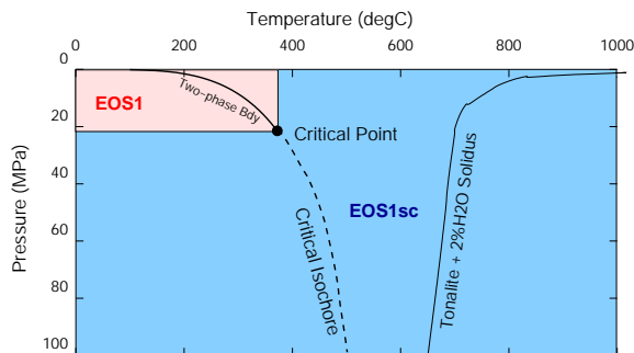
Figure 3: P-T Validity Range of eos1 (pink shaded area, Pruess et al. , 1999) and EOS1sc (blue area). Liquid-vapor solidus of hydrous tonalite magma with 2 wt% H 2 O shown to indicate typical magmatic conditions (Whitney, 1975). Dashed line shows approximate location of critical isochore (line of density equal to density at the critical point).
