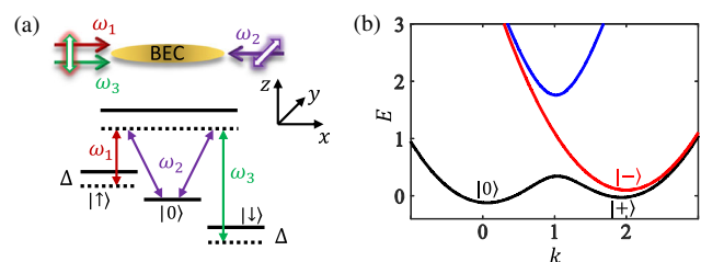
FIG. 1. (a) Top: Experimental scheme to generate STMC in a BEC. Bottom: Raman transitions between three hyperfine spin states with detuning \Delta . (b) Single-particle band structure for Raman strength \Omega = 0.5 and detuning \Delta = 0.1 . The (dominant) spin components |0\rangle and |\pm\rangle = (1/\sqrt{2})(|\uparrow\rangle \pm |\downarrow\rangle) are indicated around the corresponding band minima.
