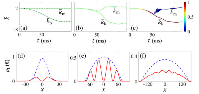
FIG. 4. (a)–(c) Averaged momentum \bar{k}_m ( \bar{k}_b ) and percentage population (color bar) of atoms in the middle (bottom) band. The thin dashed line in (a) shows the band minima. (d)–(f) The initial (dashed line) and final (solid line) spin density \rho_{\uparrow} corresponding to (a)–(c), respectively. The interactions are (g_0\bar{n}, g_2\bar{n}) = (0, 0) , (0.5, 0) , and (4, -0.2) for (a), (b), and (c), respectively. Other parameters are T = 100 ms, \Delta = -0.05 , and \Omega_f = 0.7 .
