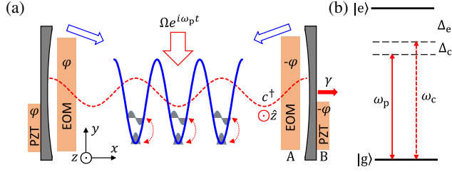
FIG. 1. (a) Schematic of the experimental setup. The cavity is pumped by an external transverse laser (red block arrow), with the cavity mode (red line) shaken by the two EOMs or PZT-driving mirrors. A BEC is prepared inside the cavity with a background lattice (blue line) generated by additional lasers (blue block arrows). The shaken cavity mode may induce interband couplings (dotted arrows) when the band gap matches the shaking frequency. (b) Energy levels of the atom and detunings of the cavity mode and pumping laser.
