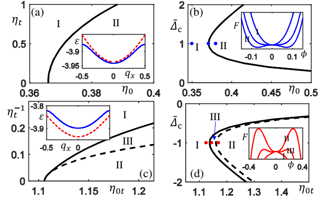
FIG. 3. (a), (b) Phase diagrams for dominant intrasideband coupling, with (a) \tilde{\Delta}_c = 1 and (b) \eta_t = 0.5 . I (II) represents the normal (superradiant) phase. (c), (d) Phase diagrams for dominant intersideband coupling, with (c) \tilde{\Delta}_c = -1 and (d) \eta_t^{-1} = 0.1 , \eta_{0t} = \eta_0\eta_t . III represents the hysteresis region. The insets in (a) and (c) show the s_0 -band dispersion in the normal (red dashed line) and superradiant phases (blue solid line). The three blue (red) dots in (b) [(d)] belong to different phases, and they mark the points where the free energy curves are plotted in the inset. The parameters are v_e = -6 , \omega = 4.8 , and \gamma = 2 (with energy unit E_R = \hbar^2 k_0^2 / 2m ), and atom-atom interaction is neglected.
