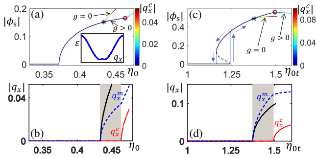
FIG. 4. (a), (c) Superradiant order parameters and condensate momenta versus \eta_0 and \eta_0 t . Stars and circles mark the transition points between zero and finite condensate momenta for g = 0 and g > 0 , respectively. The inset of (a) shows the band structure for |q_x^m| > 0 . A clear hysteresis loop appears in (c) with solid lines (dashed lines) corresponding to stable (unstable) steady-state solutions. (b), (d) Difference between q_x^c (red dotted line) and q_x^m (blue dashed line) for g > 0 . In the gray region, bosons are condensed into the local band maximum at q_x = 0 . The black solid line shows q_x^m = q_x^c for g = 0 . (a), (b) [(c), (d)] correspond to dominant intrasideband (intersideband) couplings with \Delta_c = 1 , \eta_t = 0.5 and g\bar{n} = 0.02 ( \Delta_c = -1 , \eta_t^{-1} = 0.15 and g\bar{n} = 0.1 ). \bar{n} = N_a/L is the average density, with L as the system size. Other parameters are the same as in Fig. 3.
