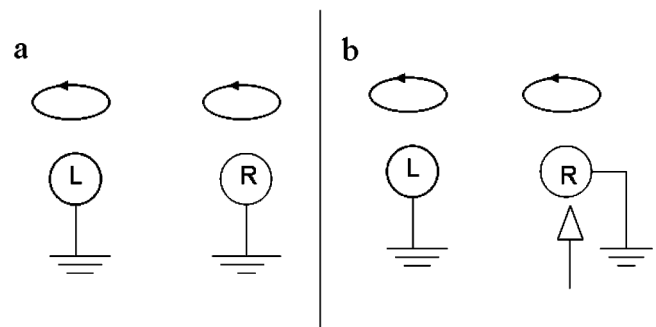
FIG. 1. (a) Two quantum dots in tunneling contact with two vortices. (b) A quantum dot and a STM tip in tunneling contact with two vortices.
