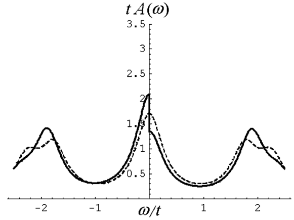
FIG. 2. The tunneling curves for J = 0.5t . Dashed curve, \epsilon_L = 0 ; solid curve, \epsilon_L = t .
