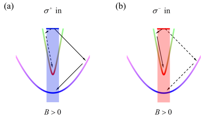
Supplementary Figure S2 | Schematic of the exciton formation processes. The shaded region denotes the light cone, and blue and red colors denote the (a) \sigma^+ or (b) \sigma^- excitation respectively. The purple and green colors on the dispersion curves denote respectively linear polarization transverse or longitudinal to the momentum. For B > 0 , comparing the valley-conserving exciton formation processes (solid arrows), the one under \sigma^- excitation is facilitated in the upper exciton branch by its steeper dispersion, and is therefore more efficient than the one under \sigma^+ excitation which requires larger momentum transfers by scattering in the lower branch to reach the light cone. Similarly, comparing the valley-flipping exciton formations (dashed arrows), the one under \sigma^+ excitation is more efficient than that under \sigma^- excitation.
