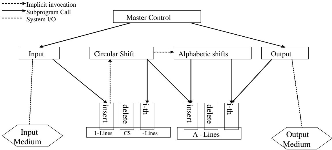
Architecture 4: Implicit Invocation
