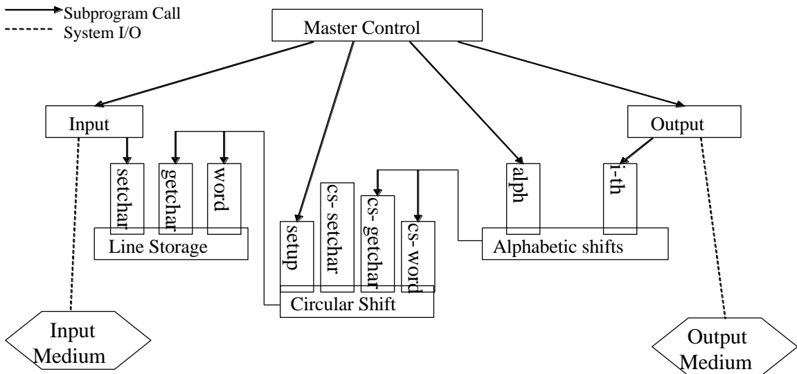
Architecture 3: Abstract Data Type
