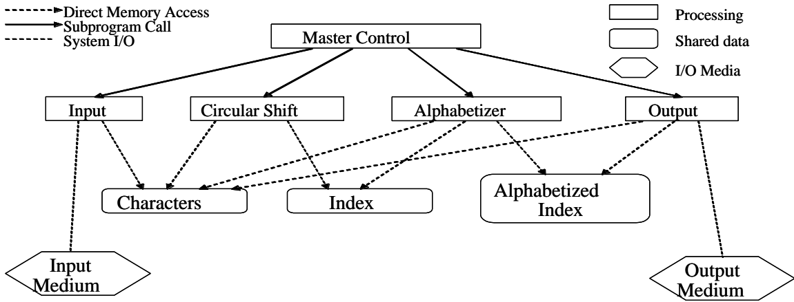
Architecture 2: Shared Data
