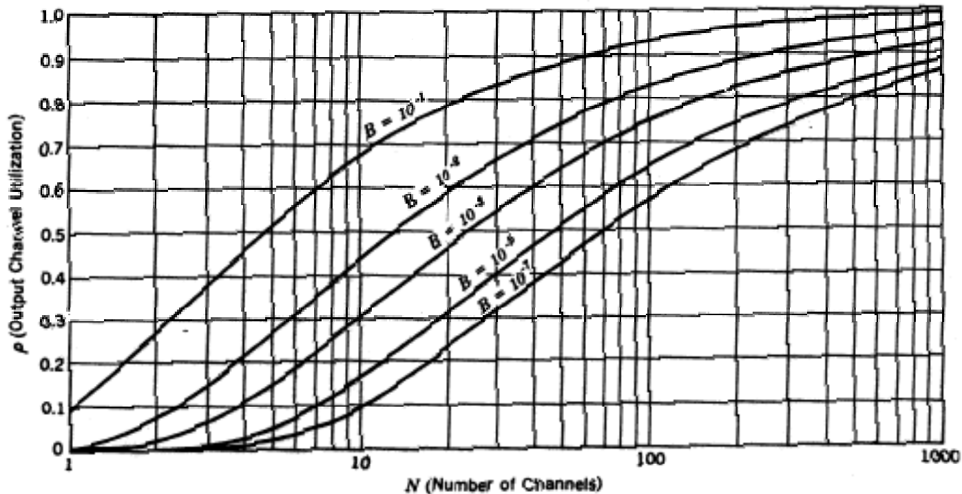
Figure 10.5. Output channel utilization of lost calls cleared system.
