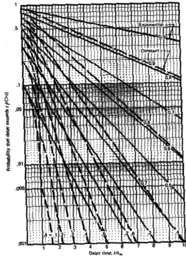
Figure 10.18. Delay probabilities of single-server systems (exponential and constant service times).
