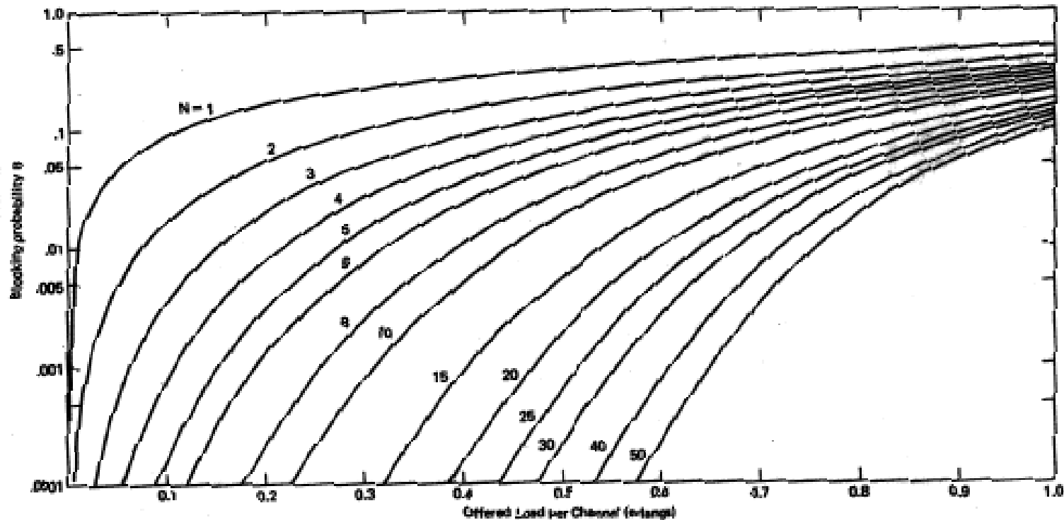
Figure 10.4. Blocking probability of loss calls cleared system.
