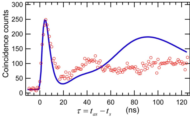
Fig. 4. (Color online) Zoomed view of Fig. 2(b) comparing the experimental data (circles) and the theoretical curve (solid curve). Optical depth=62.
