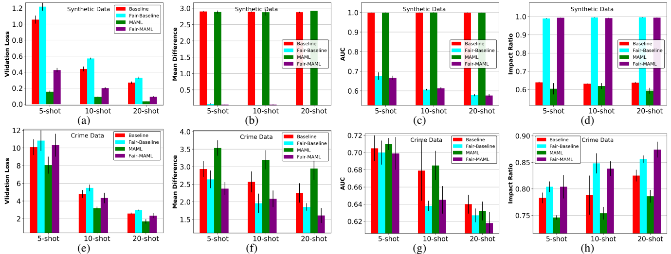
Fig. 5: Experiment results of controlling biases and fairness generalization to unseen data for meta-learning regression problem.
