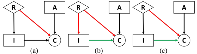
Fig. 2: CBN representing a hypothetical crime forecasting process with three possible scenarios, where red and green paths are used to indicate unfair and partially-unfair links, respectively.
