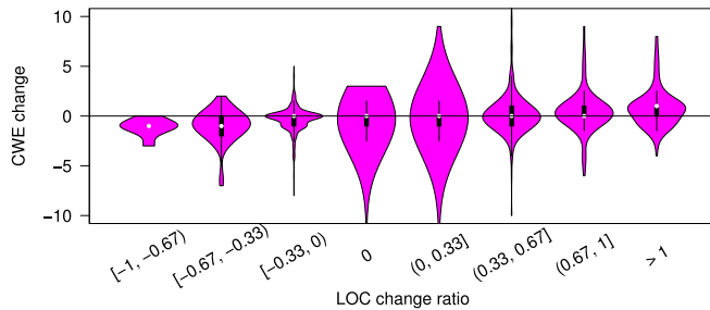
Fig. 6. The distribution of the change of CWE instances number across different ranges of LOC change ratio. The negative CWE change occurs within the improved Code w . The zero CWE change occurs within the unchanged Code w . The positive CWE change occurs within the deteriorated Code w .
