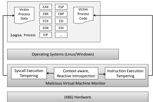
Figure 3: Architecture Overview of Our Attack.
