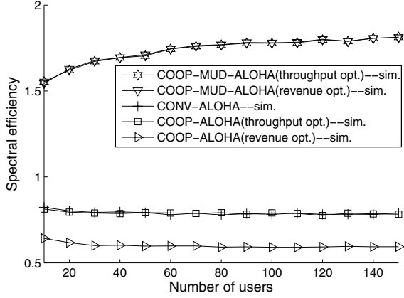
Fig. 6. Spectral efficiency comparison for the collision model
