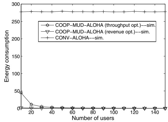
Fig. 12. Energy consumption comparison for the MPR model
