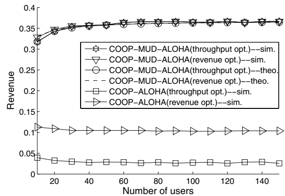
Fig. 5. Revenue comparison for the collision model
