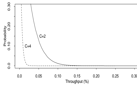
Figure 16: Upper bound on probability that a connection's fraction of marked packets is more than C times the expected number, given 100 total marked packets.
