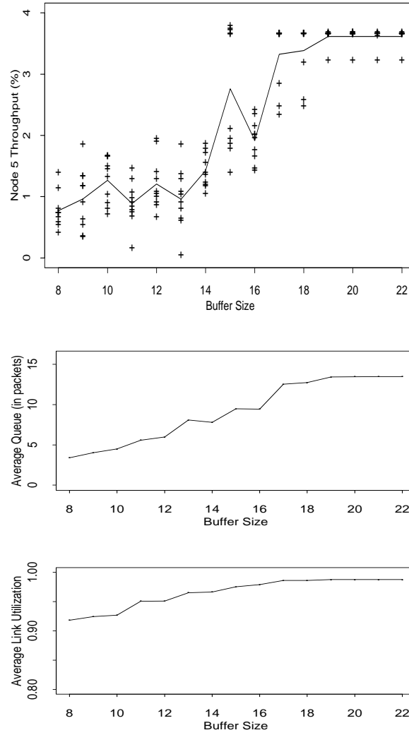
Figure 13: Simulations with Random Drop gateways.
