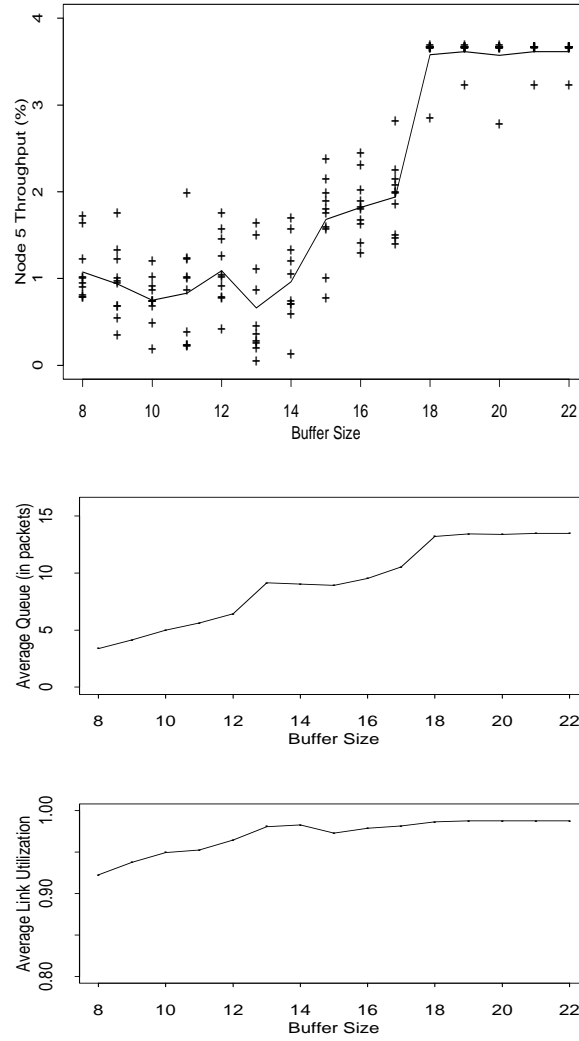
Figure 12: Simulations with Drop Tail gateways.
