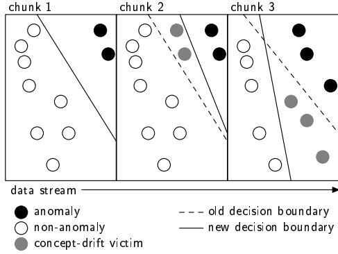
Fig. 1. Concept drift in stream data
