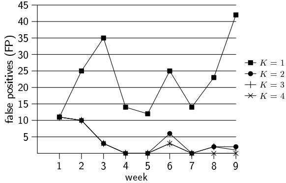
Fig. 6. Distribution of false positives
