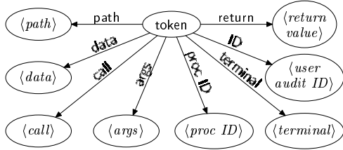
Fig. 5. A token subgraph
