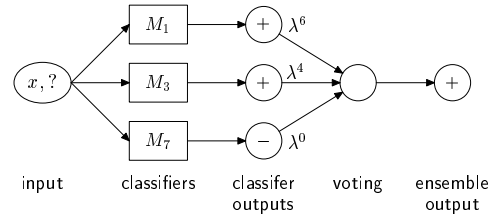
Fig. 2. Ensemble classification
