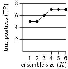
Fig. 10. The effect of K on TP rates for fixed q = 4 on dataset A
