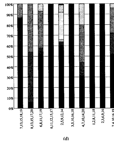
Figure 9: Resulting color for the faulty statements (left) and nonfaulty statements (right) in multiple fault versions across all tests suites.
