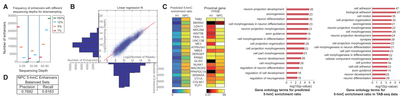
Fig. 5. 5-hmC status prediction in enhancers. (A) Sequencing depth across cytosines in enhancers after downsampling. (B) Log-log linear regression fit (mapped read count versus sequencing depth across cytosines) in NPC enhancers. (C) Heatmap of predicted 5-hmC enrichment ratio and proximal gene expression for enhancers with highest predicted gain in 5-hmC enrichment ratio (NPC versus H1). GO term enrichment for genes with highest 5-hmC enrichment ratio (NPC versus H1) using predictions and TAB-seq data. (D) 5-hmC status prediction in NPC enhancers
