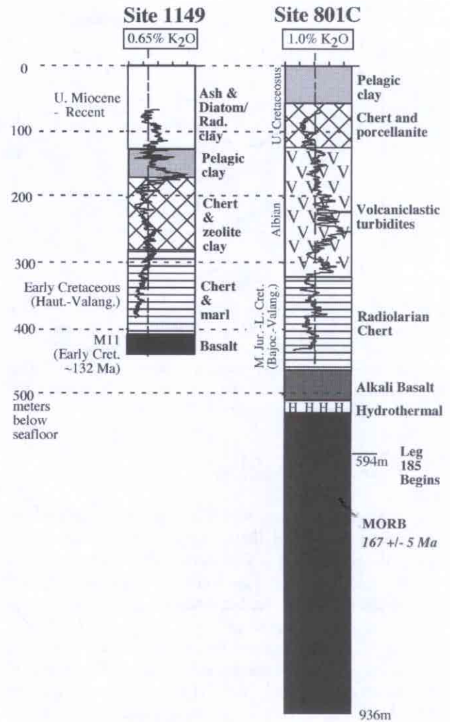
Figure 7. ODP sites 801C and 1149, locations shown on Figure 3. 801C is thought to be representative of sediments being subducted beneath the Marianas and 1149 of those going down beneath Izu-Bonin. Superimposed on simplified lithological columns are K contents determined using the natural gamma down hole logging tool. Note that enrichments in K and other incompatible elements in sediments being subducted beneath the Mariana arc is largely due to the thick sequence of Albian (Cretaceous) volcanics. http://www-odp.tamu.edu/publications/185_IR/VOLUME/CHAPTERS/IR185_04.PDF
