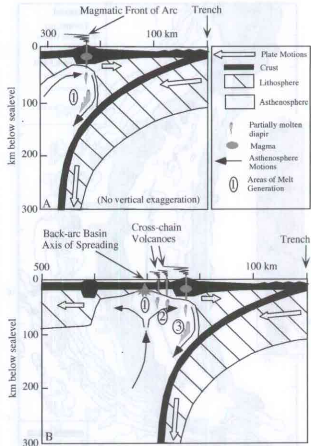
Figure 25. Conceptual models for evolution of the Subduction Factory from one lacking an actively spreading back-arc basin (A) to one associated with back-arc spreading (B). Note that magma generation and migration beneath the magmatic front occurs in a region of mantle downwelling, whereas that beneath the back-arc basin spreading axis occurs in a region of mantle upwelling. Note in (B) the multiple melting opportunities for mantle rising beneath the back-arc basin, with melt generation beneath the spreading axis (1), beneath cross-chains (2) and beneath the magmatic front (3). The IBM arc system presents all of these stages, with the Bonin segment now acting as an unrifted arc (A) whereas the Mariana segment is an outstanding example of an arc associated with back-arc spreading (B). The Izu segment represents an intermediate situation, where rifting is underway but has not proceeded to seafloor spreading.
