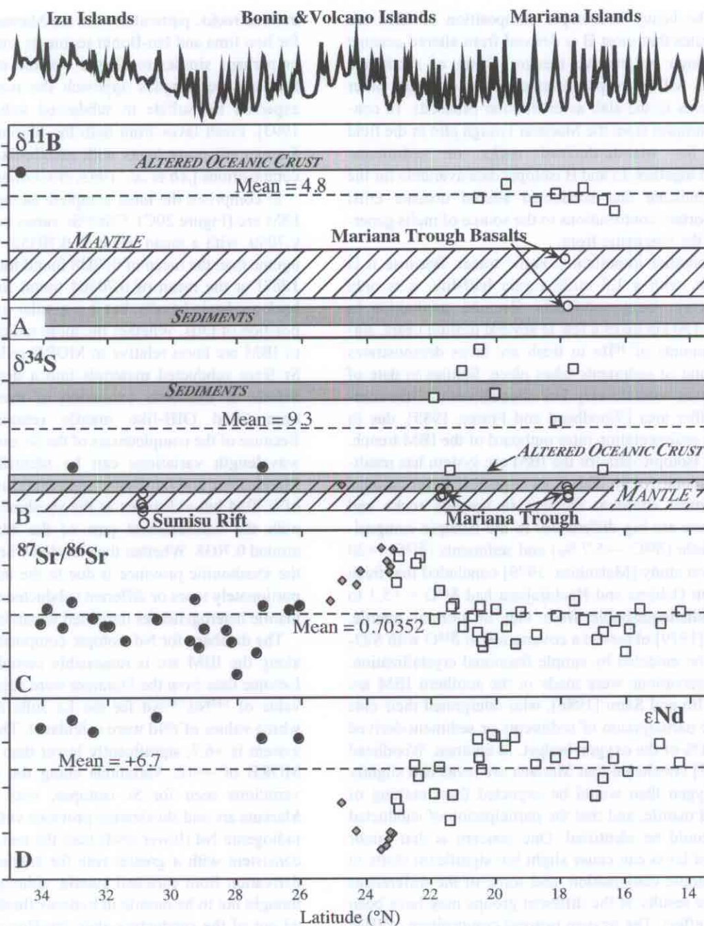
Figure 20. Isotopic variations along the IBM arc. Symbols are the same as in Figure 17 (filled circles: Izu-Bonin; diamonds: Shoshonitic Province; open squares: Mariana). (A) B isotopic variations; data for IBM arc after Ishikawa and Nakamura [1994] and Ishikawa and Tera [1999]; data for Mariana Trough basalts after Chaussidon and Jambon [1994]. Isotopic composition of altered oceanic crust, sediment, and mantle are from Ishikawa and Tera [1999]. (B) S isotopic composition of IBM arc lavas, Mariana Trough, and Sumisu rift lavas. Data for IBM arc lavas from Alt et al. [1993], Ueda and Sakai [1984], and Woodhead et al. [1987]; Data for ten Mariana Trough basalts are from Alt et al. [1993]; for 7 Sumisu Rift lavas from Hochstaedter et al. [1990a]. Fields for sediments, altered oceanic crust, and mantle are from Alt et al. [1993]. (C) Sr isotopic data for IBM arc lavas, normalized to E&A \text{SrCO}_3 ; data sources described in text. (D) Nd isotopic data for IBM arc lavas, adjusted to a common value for the La Jolla Nd standard; data sources described in text.
