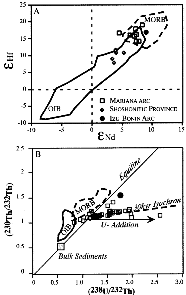
Figure 23. (A) Hf-Nd isotopic variations for the IBM arc system, data from [Pearce et al. , 1999; White and Patchett, 1984; Woodhead, 1989] (Vervoort, personal communication, 2000). Fields for OIB and MORB are from Vervoort et al. [1999] and define the mantle array. (B) U-Th disequilibrium data for IBM arc lavas. Data are not averaged for each edifice. Data from Elliott et al. [1997], Gill and Williams [1990], McDermott and Hawkesworth [1991], Newman et al. [1984], and Reagan (personal communication, 2000).
