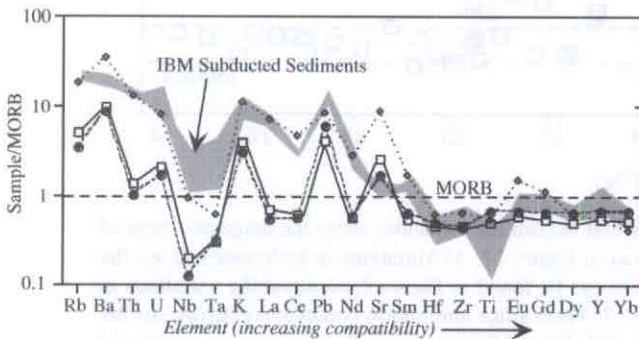
Figure 19. Incompatibility plot for lavas from along the front of the IBM arc. Typical compositions for the Mariana arc (GUG-9 of Elliott et al. [1997]; 51% SiO 2 ) and Shoshonitic province (54H of Peate and Pearce [1998]; 47.8% SiO 2 ) are plotted, along with a mean calculated for Izu arc mafic lavas (51.6% SiO 2 [Taylor and Nesbitt, 1998]). Symbols are the same as in Figure 17 (filled circles: Izu-Bonin; diamonds: Shoshonitic Province; open squares: Mariana). Composition of MORB and element order is after N-MORB of Hofmann [1988]. Grey field outlines the composition of IBM subducted sediment, from Figure 8.
