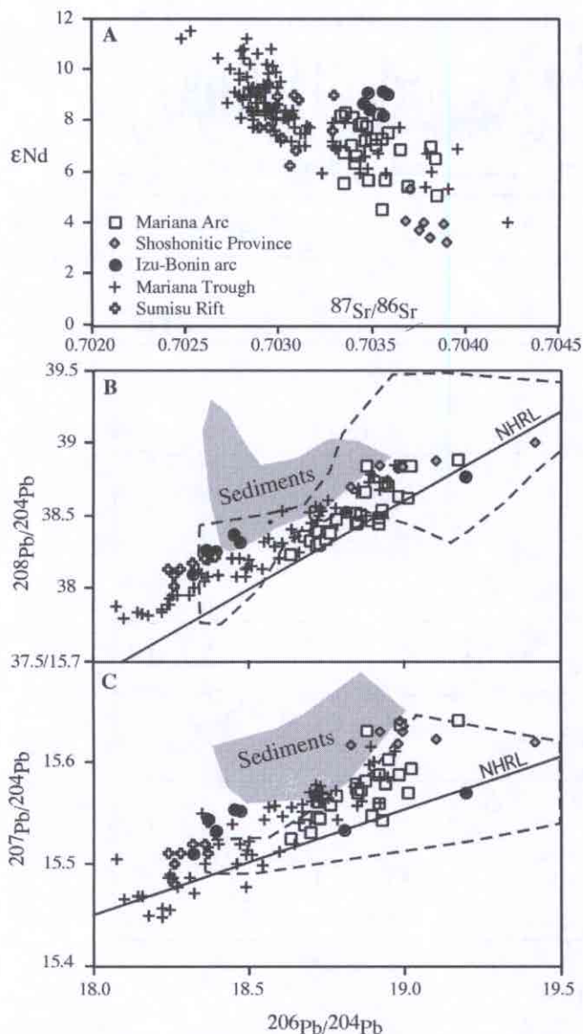
Figure 21. Isotopic composition of Sr, Nd, and Pb for IBM arc lavas, including Sumisu Rift and Mariana Trough basalts. Data for IBM arc are averages for individual volcanoes, data for Sumisu Rift and Mariana Trough are individual analyses. Fields for sediments (shaded) and W. Pacific off-ridge volcanics (dashed), taken from Figure 9, are shown in B and C. Location of these diagrams is shown with dashed boxes on Figure 9. The Northern Hemisphere Reference Line (NHRL [Hart, 1984]) is shown for comparison.
