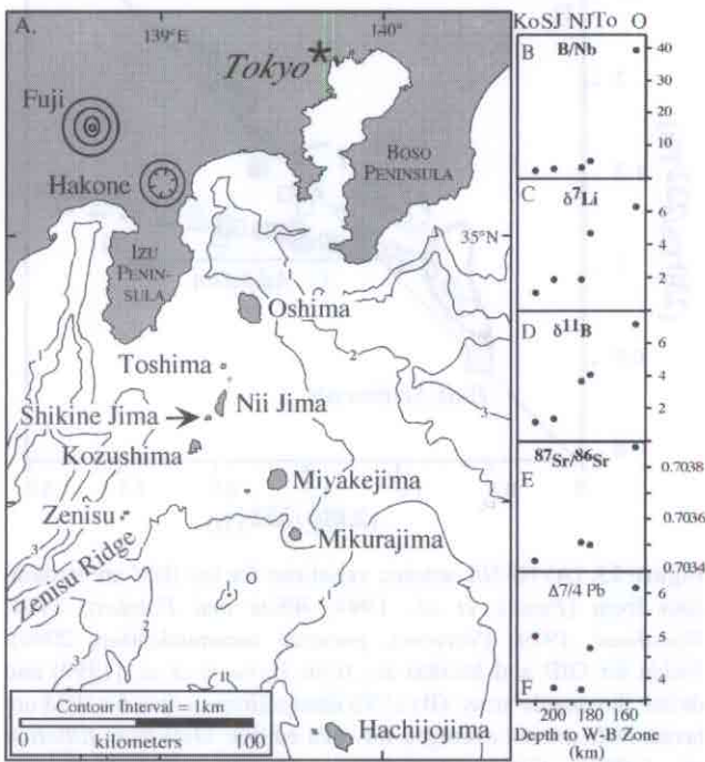
Figure 24. A) Locality map for the northern IBM arc system and the Zenisu cross-chain. B-F) plot volcano-means for parameters sensitive to fluid input (B) or contributions from the subducted slab (C-F) vs. depth to the Wadati-Benioff zone. B) Variations of B/Nb vs. depth to the Wadati-Benioff Zone. Islands Oshima (Os), Toshima (To), Nii Jima (NJ), Shikine Jima (SJ), Kozushima (Ko); C) Variations of \delta^7\text{Li} vs. depth to the Wadati-Benioff Zone; D) Variations of \delta^{11}\text{B} vs. depth to the Wadati-Benioff Zone; E) Variations of ^{87}\text{Sr}/^{86}\text{Sr} vs. depth to the Wadati-Benioff Zone; F) Variations of \Delta^{7/4}\text{Pb} vs. depth to the Wadati-Benioff Zone. Notice the decrease in all parameters sensitive to subducted inputs with greater depth to the seismic zone. Data are from Ishikawa and Nakamura, [1994], Moriguti and Nakamura [1998], and Notsu et al. [1983].
