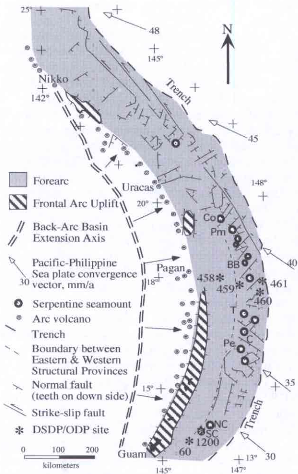
Figure 15. The IBM forearc, between 13° and 25°N, shown in gray. Generalized structural features and location of serpentinite mud volcanoes are taken from Stern and Smoot [1998]. Dashed line marks the boundary between rough and smooth terrains of Stern and Smoot [1998], or between Eastern and Western Structural Provinces of Mrozowski and Hayes [1980]. Arrows radiating out from the back-arc basin extension axis show how differential extension causes decreasing radius of curvature of the arc, leading to stretching of the forearc along strike. Location of DSDP sites 60, 458, 459, 460, 461, and 1200 are shown. ODP sites 778-781 are centered on Chamorro Seamount. Names of serpentinite mudvolcanoes, after Fryer et al. [1999] from south to north: South Chamorro, SC; North Chamorro, NC; Blue Moon, BM; Peacock, Pe; Celestial, C; Turquoise, T; Big Blue, BB; Pacman, Pm; Conical, Co.
