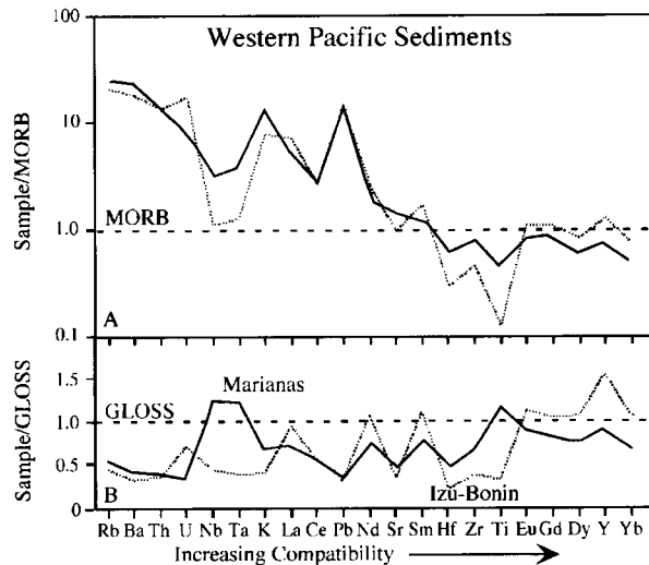
Figure 8. Chemical composition of sediments being fed into the IBM Subduction Factory. Composites for sediments outboard of Izu-Bonin (dotted line) and Mariana (solid line) are after Plank and Langmuir [1998], (A) normalized to abundances in MORB [Hofmann, 1988] and (B) normalized to Global Subducting Sediments (GLOSS; [Plank and Langmuir, 1998]).
