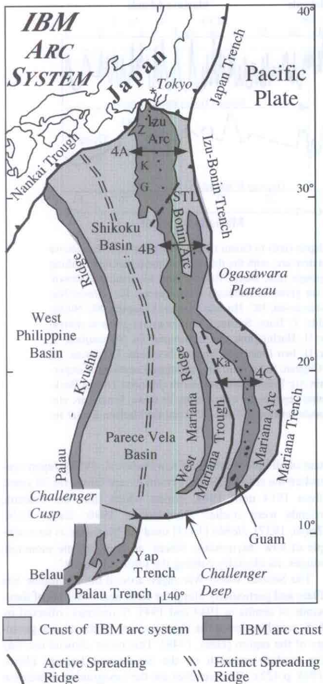
Figure 1. Generalized locality map for the Izu-Bonin-Mariana Arc system. Dashed line labeled STL = Sofugan Tectonic Line. Traverse shown in Figure 2 follows the magmatic arc from Japan through the Izu, Bonin, and Mariana magmatic arcs. Locations of profiles shown in Figure 4 are shown and labeled 4A, 4B, and 4C. Location of cross-chains is shown, with Zenisu (Z) at the far north, Kan'ei (K) and Genroku (G) farther south in the Izu arc, and Kasuga (Ka) in the Marianas.
