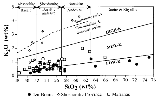
Figure 17. Potassium-silica diagram for the mean composition of 62 volcanoes along the magmatic front of the IBM arc system. Data sources discussed in text. Names for rocks indicated for calc-alkaline and tholeiitic series below the double arrows, above the double arrows for the shoshonitic series.
