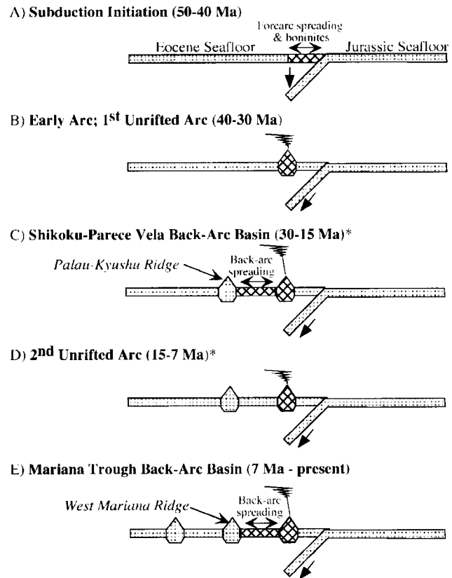
Figure 5. Simplified history of the IBM arc system. Shaded areas are magmatically inactive, cross-hatched areas are magmatically active.
