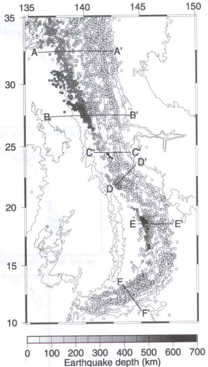
Figure 10. Map view of bathymetry and seismicity in the Izu-Bonin-Mariana Subduction Factory using the earthquake catalog of Engdahl et al. [1998]. Circles denote epicentral locations; lighter circles represent shallower events, darker circles represent deeper events. Black lines denote cross-sectional areas depicted in Figure 11. Large variations in the seismic structure of the region are evident.
