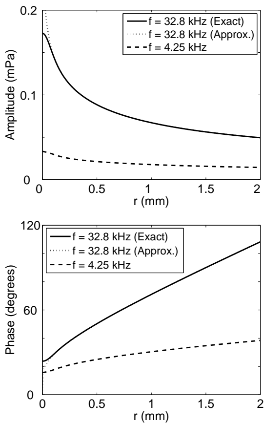
Fig. 2 The amplitude (top) and phase (bottom) of the acoustic pressure wave as a function of the radial distance r from the center of the laser beam. The solid and dashed curves show the results for the 32.8 kHz and 4.25 kHz modulation frequencies, respectively, as computed using the exact formulae (8)–(10). The dotted curves show the result for the 32.8 kHz modulation frequency computed using the approximation (14) of (10). The solid and dotted curves overlap for r > 0.1 mm.
