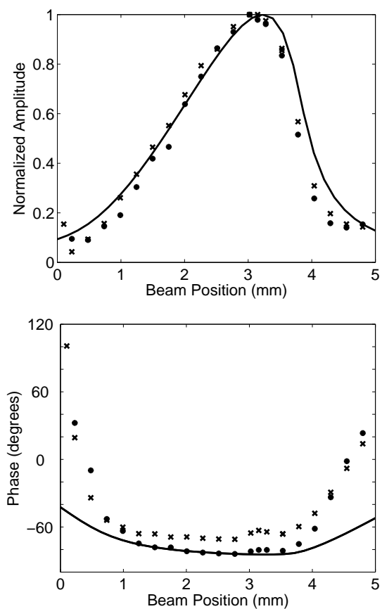
Fig. 3 Normalized amplitude (top) and phase (bottom) of the piezoelectric current as functions of the vertical position, y_0 , of the laser beam for a QEPAS sensor with a 32.8 kHz tuning fork. The theoretical results are shown with solid lines, and the experimental data measured at 450 Torr and 60 Torr are shown with dots and crosses, respectively. These results are from the first set of experiments using the \text{NH}_3:\text{N}_2 mixture.
