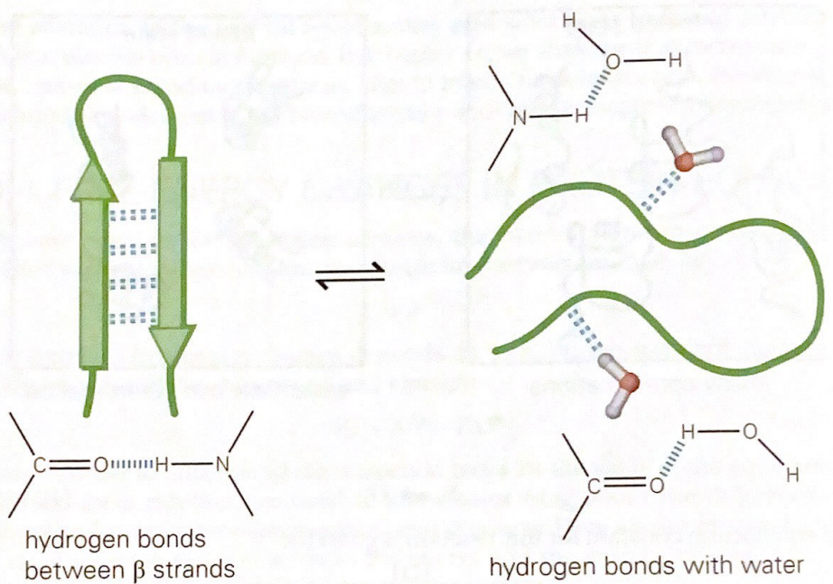
Figure 10.14 Hydrogen bonds in protein folding. In a folded protein structure, most hydrogen-bonding groups interact with other groups within the protein. When the protein unfolds, these groups interact with water instead. The difference in hydrogen-bonding energy between the two situations is close to zero, but the hydrogen bonds in the folded protein might have slightly lower energy if the groups are favorably oriented.
