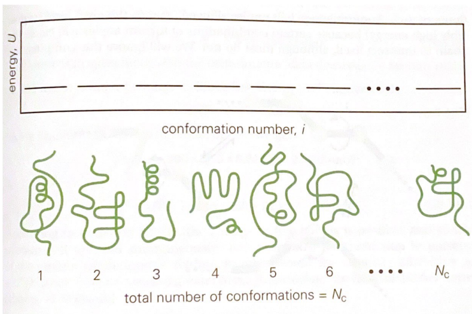
Figure 10.17 All unfolded conformations are equally probable. We assume that there are N_c unfolded conformations. The energy of each conformation is shown in this diagram, along with the structure. Because all of the energies are the same, the probability of finding any of these conformations is the same.
