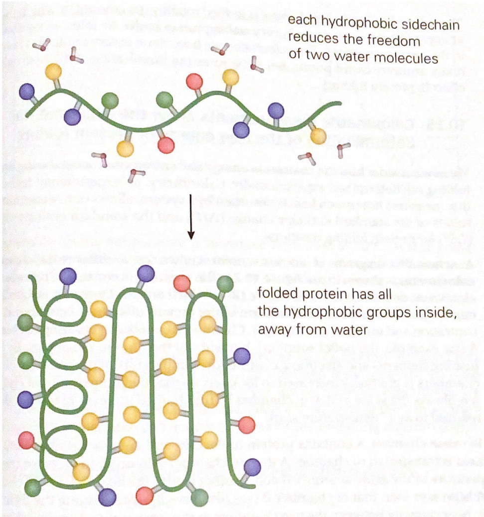
Figure 10.23 Hydrophobic groups in protein folding. In our simple model, we assume that half of the protein sidechains are hydrophobic, and that all of them are buried in the folded protein. In the unfolded state, each hydrophobic sidechain interacts with two water molecules. We assume that these water molecules are the only ones affected by the unfolded protein.
