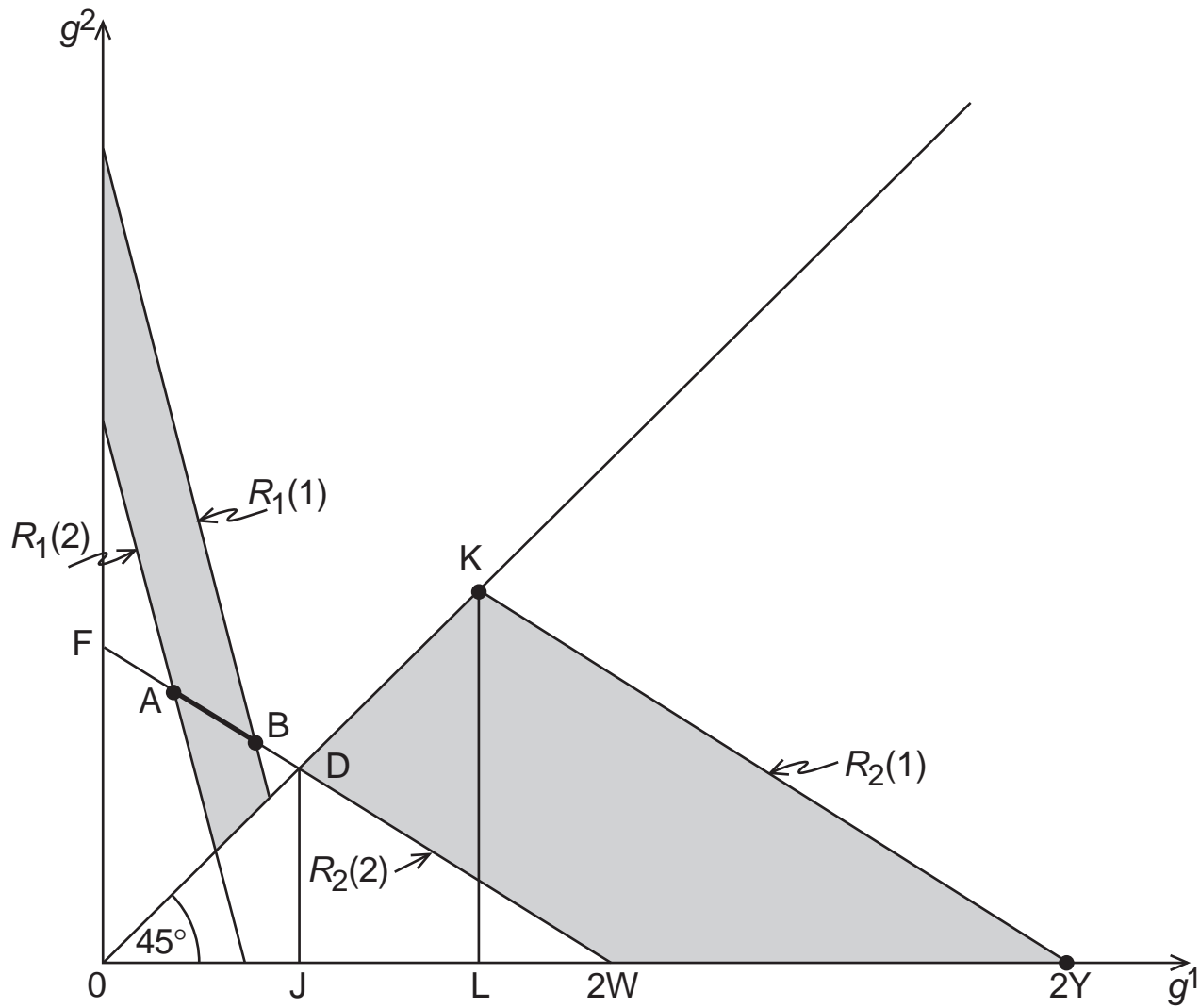
Figure 2. Nash reaction correspondences
