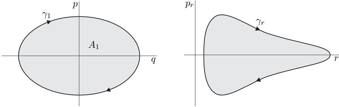
FIGURE 2. Periodic orbits on the q - p and r - p_r planes.
