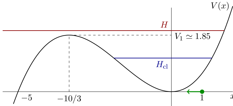
FIGURE 3. Potential (39) with m = 1 , \omega = 1 , c = 1/10 ; H_{\text{cl}} is the classical Hamiltonian and H is the semiclassical Hamiltonian (20) with initial condition (40). H_{\text{cl}} < V_1 < H implies classical trajectory is trapped but semiclassical trajectory may escape through the potential barrier. The green dot and arrow on the x -axis indicate the initial position and velocity of the particle.
