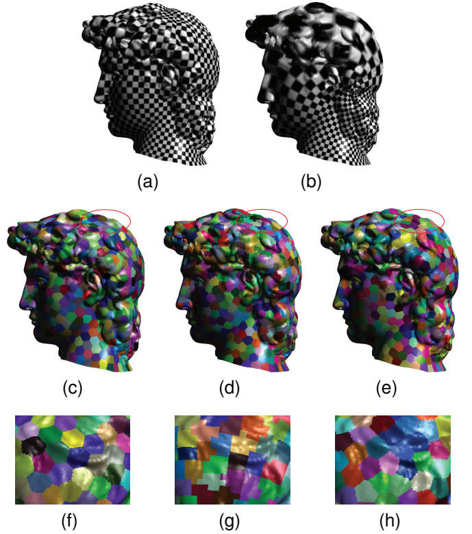
Fig. 12. (a)&(b) Comparison of two different parameterizations of David Head. (c) the CVTs computed using the parameterization in (a) with a 512 \times 416 geometry image; (d) the CVTs computed using the parameterization in (b) with a 512 \times 191 geometry image; and (e) the CVTs computed using the parameterization in (b) with a 2048 \times 765 geometry image. (f)-(h) are enlarged top views of the circled part.
