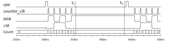
Fig. 10: Partial dynamic reconfiguration demonstration
