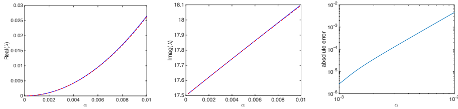
Figure 1. Small dissipation results at an edge bifurcation. Left: The real part of the bifurcating eigenvalue as a function of \alpha . The results obtained using our method are shown with the blue solid line, and the results obtained using Equation (11) with \lambda_e = i(\phi_0 + m\alpha) are shown with the red dashed line. Center: The imaginary part of the same eigenvalue. Right: The distance between the eigenvalues obtained using the two methods.
