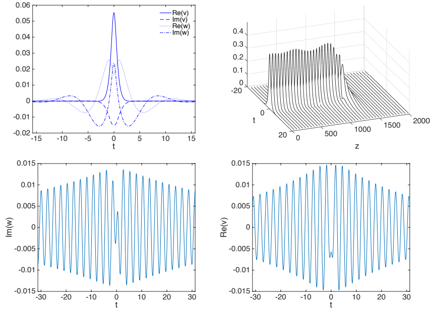
Figure 4. Upper left: The eigenfunction of the unstable eigenvalue, \lambda_+ , when D = 0.2 . Upper right: Evolution of a perturbation of the stationary solution by the unstable eigenfunction in the upper left panel. Lower left: The imaginary part of the w -component of the eigenfunction with eigenvalue, \lambda_{\mathfrak{R},2} , when D = -0.026 . Lower right: The real part of the v -component of the eigenfunction with eigenvalue, \lambda_{\mathfrak{R},1} , when D = -0.026 .
