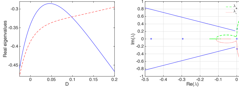
Figure 5. Left: The real eigenvalues, \lambda_{\mathfrak{R},1} (solid blue line) and \lambda_{\mathfrak{R},2} (dashed red line), as functions of D . Right: The curves of the eigenvalues, \lambda_+ (dashed green curve) and \lambda_- (dotted red curve), parametrized by D which decreases from D = 0.2 to D = -1 . The curves start in the right-half plane at D = 0.2 . The solid blue lines and symbols show the spectrum at the Hopf bifurcation point, D_{\text{cr}} = 0.047 .
